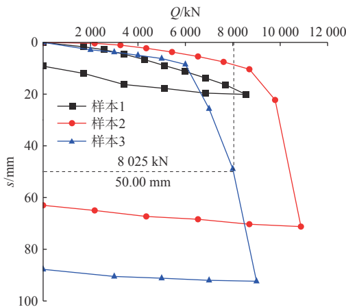
图 2 3 个样本的试桩 Q - s 曲线 Fig. 2 Q - s curves of three samples by static load test
