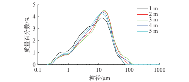
图 1 泾阳不同深度黄土粒径分布占比图 Fig. 1 Proportion of particle size distribution of loess at different depths in Jingyang
