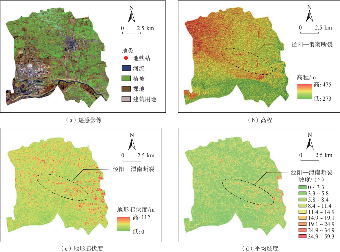
图 3 高陵区地貌特征图 Fig. 3 Geomorphic features of the hilly region
