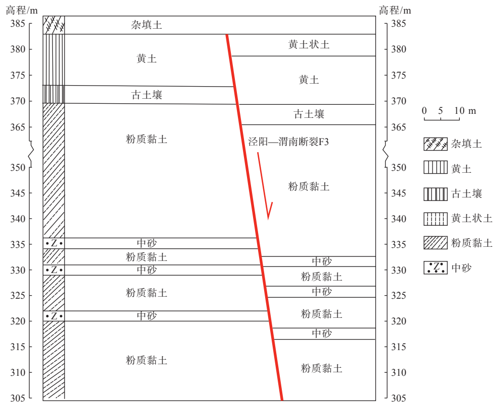
图 2 泾阳—渭南断裂工程地质简化剖面图 Fig. 2 Simplified engineering geological profile of Jingyang–Weinan fault
